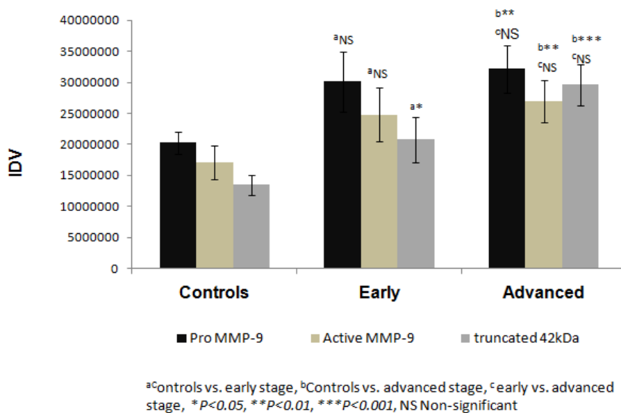
Fig-3. Expression of pro MMP-9, active MMP-9 and truncated 42 kDa MMP in early and advanced stage of disease. Values are expressed as mean ± SEM. IDV: Integrated density value
