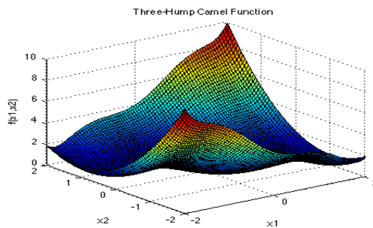
Figure-17. Three-Hump Camel Function
