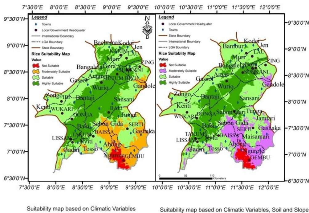
Figure-4. Rice suitability map based on the selected climatic variables.
