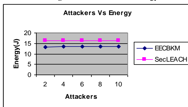
Figure-5. Attackers Vs Energy
