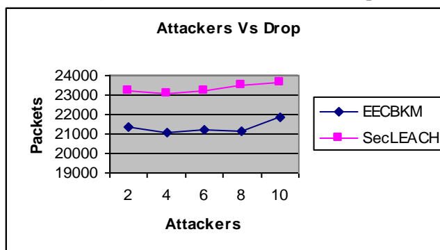
Figure-4. Attackers Vs Packet Drop
