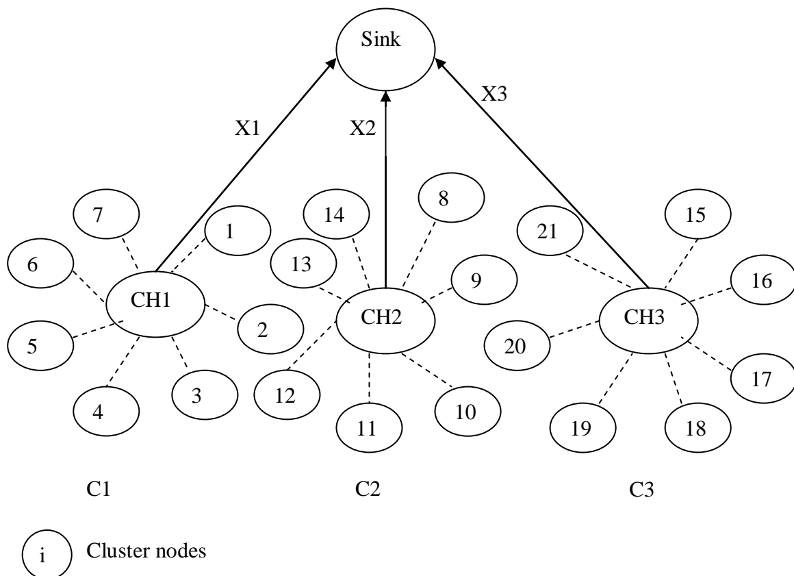
Fig-1. Clustering Architecture
