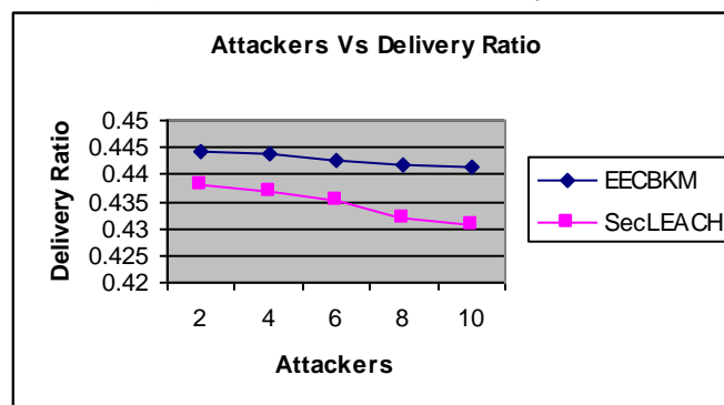
Figure-3. Attackers Vs Delivery Ratio
